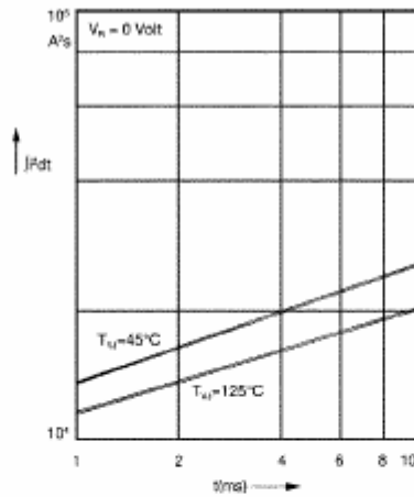
Fig. 2 J^2dt versus time (1-10 ms)
